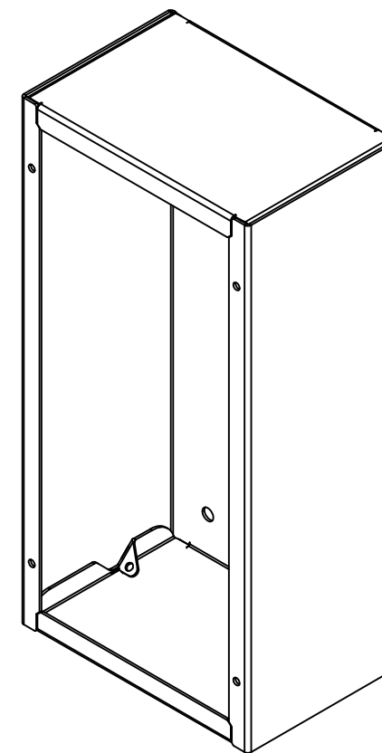
Isometric View
