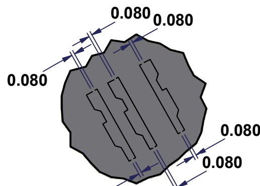
DETAIL K
