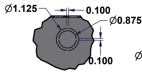
DETAIL D
