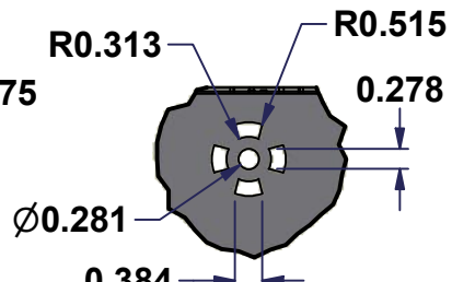
DETAIL E
