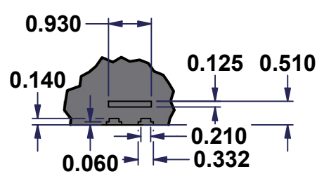
DETAIL F
