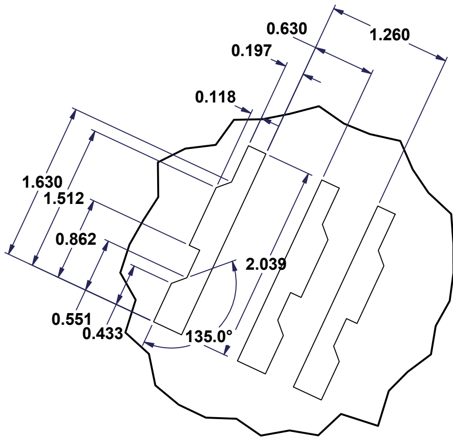
DETAIL C
