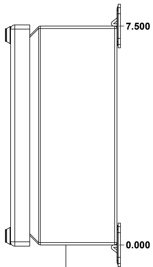
RIGHT
