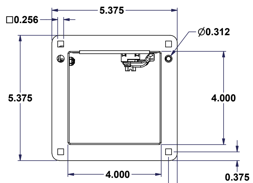
DETAIL C
