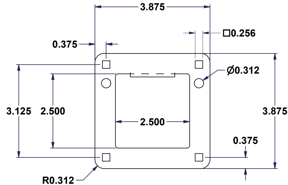
CONNECTOR Details
