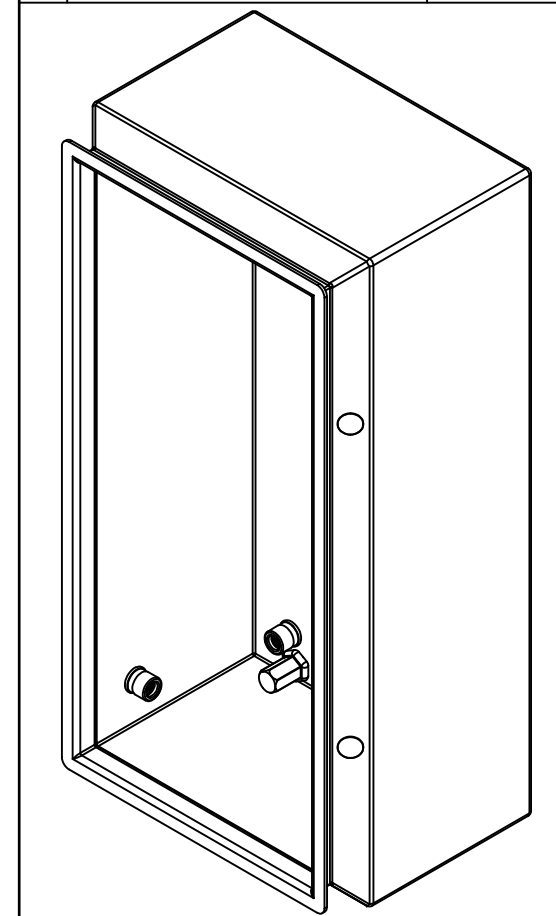
Isometric View
